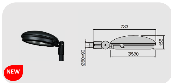
COLUMNA SEMICURVA REF:SEMIC P-900 RAL 9007+BORA H9 LED
