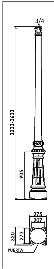
COLUMNA VILLA 3200m/m-3600m/m
