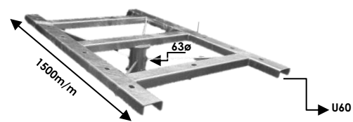
REF:CRU/H-8-1500
