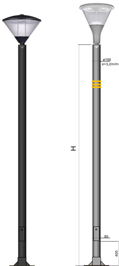
COLUMNA CILINDRICA REF: CLR/P100 DIAABOLO FUTURE
