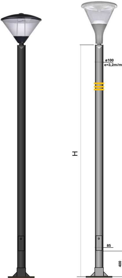
COLUMNA CILINDRICA REF: CLR/P100 DIABOLO FUTURE
