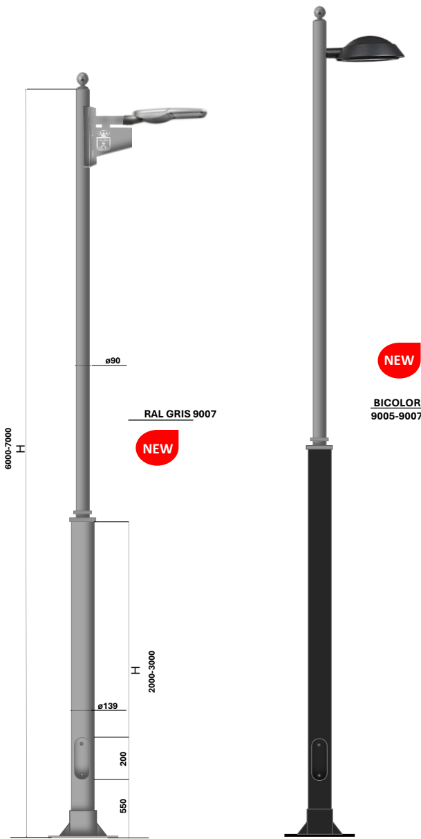
COLUMNA VARADERO P-139 RAL 9007+BORA H9 LED
