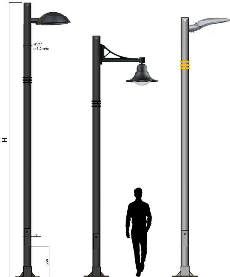
COLUMNA CILINDRICA REF: CLR/P127 ECA D-32 AROS BLACK
